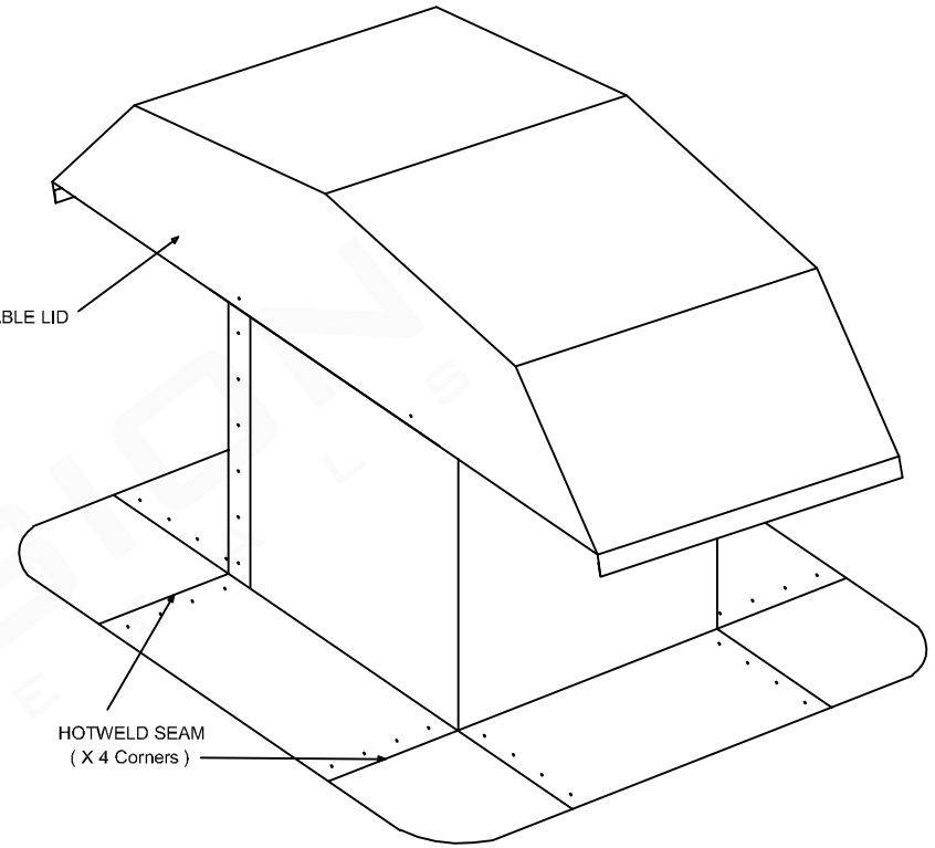
ORTHOGRAPHIC VIEW
